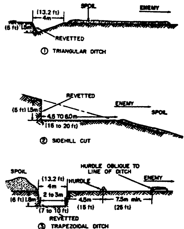
Figure 3-5. Antivehicular ditches.
